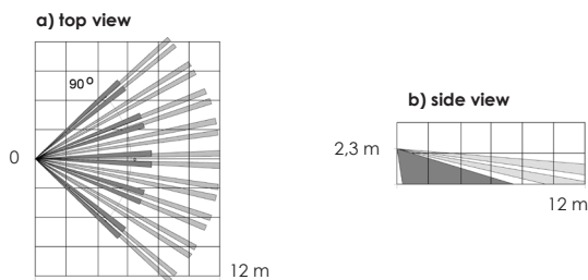
Picture 2 – Detection zone diagram
