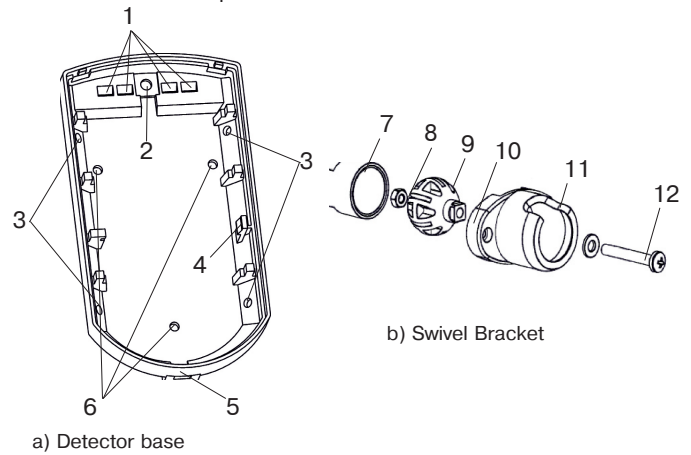
Figure 2 – Detector Base and Swivel Bracket
