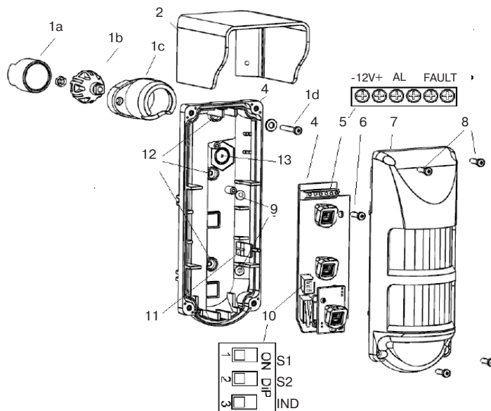
Figure 1 - The Detector Layout
