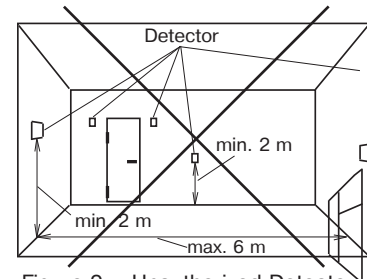
Figure 9 – Unauthorized Detector Installation Places
